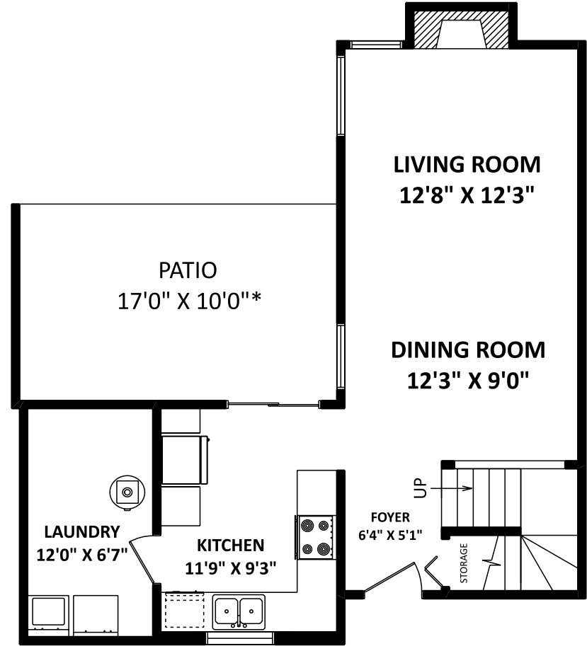
MAIN FLOOR: 582 SQ.FT.
