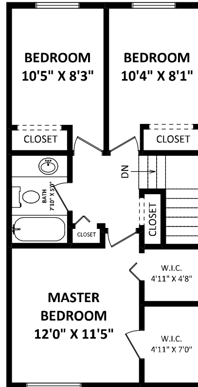
UPPER FLOOR: 595 SQ.FT.
