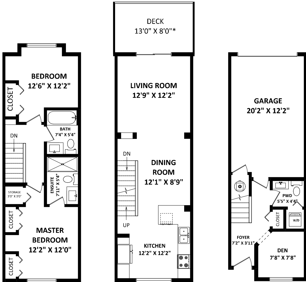
MAIN FLOOR 490 SQ.FT.
